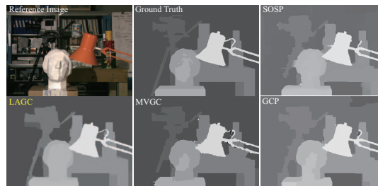
Figure 8. Stereo matching on the Tsukuba dataset. Our LAGC outperforms MVGC [14] and SOSP [37] but is slightly worse than GCP [28]. However, it better preserves edges, e.g., the left foot of the tripod. See Table 1 for numerical comparison.
