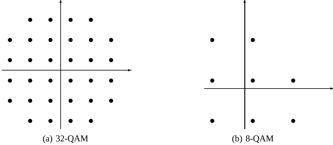
Fig. 2. Non-rectangular QAM.
