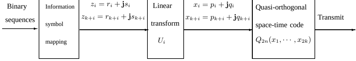
Fig. 1. Encoding of an QOSTBC.
