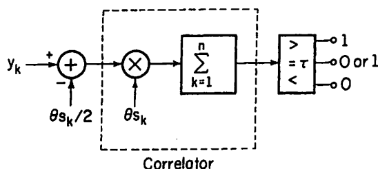
FIGURE III.E.1. Nominally optimum detector for coherent signals in Gaussian noise.
