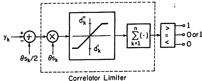
FIGURE III.E.2. Robust detector for coherent signals in nominally Gaussian noise.
