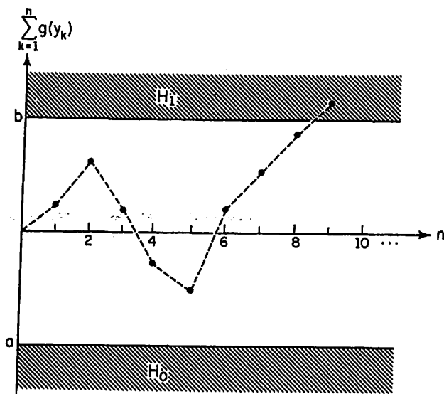
FIGURE III.D.3. Illustration of ST(a, b; g) .
