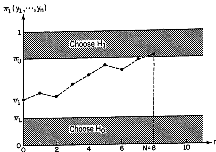
FIGURE III.D.2. Depiction of a realization of a Bayes sequential test.
