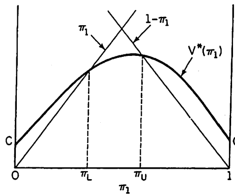
FIGURE III.D.1. Relationships yielding the Bayes sequential rule for uniform costs of errors and cost C per sample.
