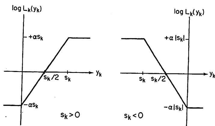
FIGURE III.B.3. Per-sample log-likelihood ratio for coherent detection in Laplacian noise.
