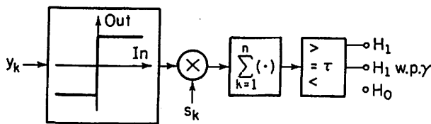
FIGURE III.B.6. Locally optimum detector for Laplacian noise.
