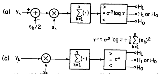
FIGURE III.B.2. Optimum detector for coherent signals i.i.d. Gaussian noise.
