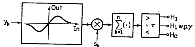
FIGURE III.B.7. Locally optimum detector for Cauchy noise.
