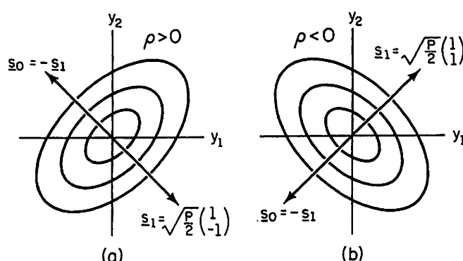
FIGURE III.B.9. Illustration of optimum signals for Gaussian noise with \Sigma_N = \sigma^2 \begin{pmatrix} 1 & \rho \\ \rho & 1 \end{pmatrix} .
