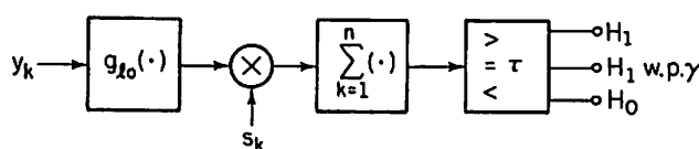
FIGURE III.B.5. Locally optimum detector structure for coherent signals in i.i.d. noise.
