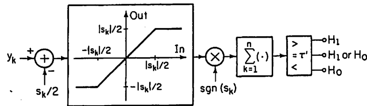
FIGURE III.B.4. Optimum detector for coherent signals in Laplacian noise.
