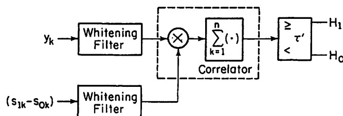
FIGURE III.B.8. Optimum detector for coherent signals in dependent Gaussian noise.
