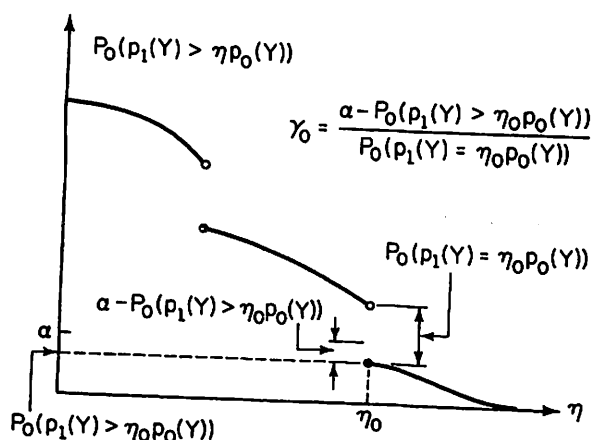
FIGURE II.D.1. Threshold and randomization for an \alpha -level Neyman-Pearson test.
