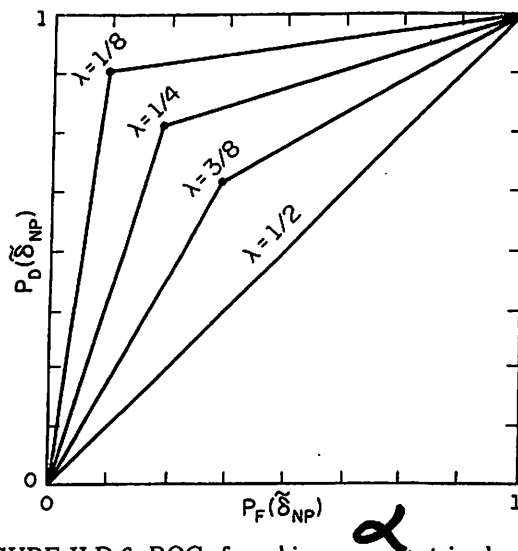
FIGURE II.D.6. ROCs for a binary symmetric channel.
