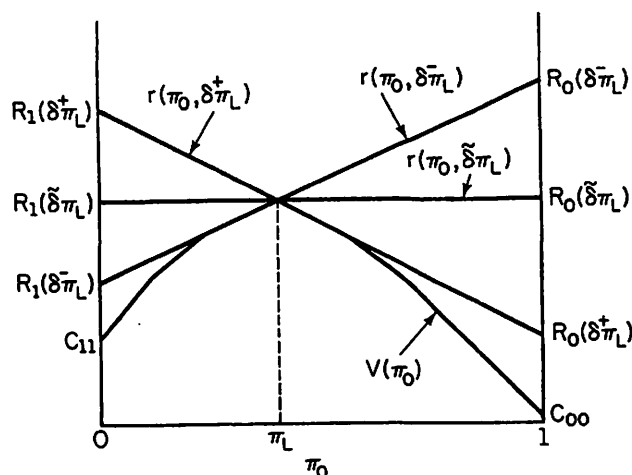
FIGURE II.C.4. Depiction of a randomized decision rule.
