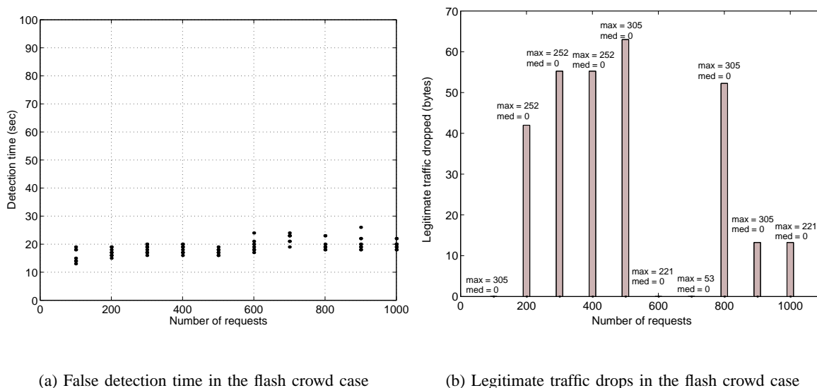
Fig. 7. False detection time and legitimate traffic drops in the flash crowd case
