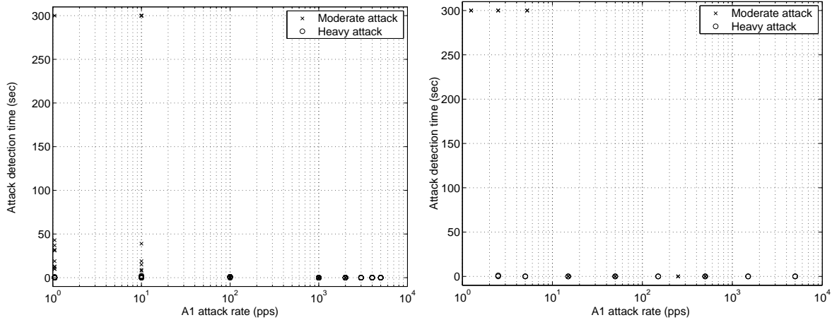
(a) Detection time of small-rate UDP attacks
