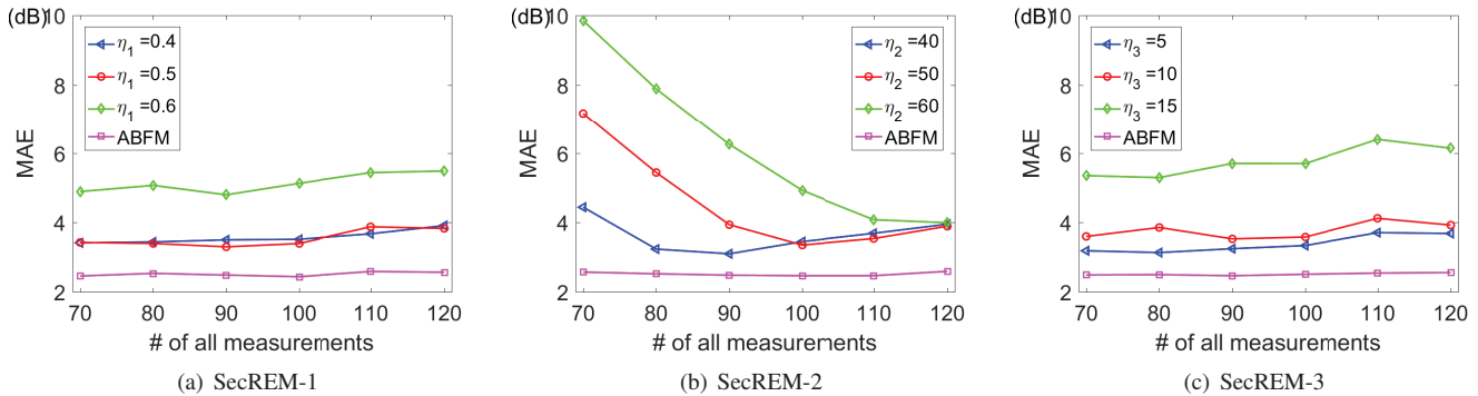
Fig. 11. MAEs of SecREM-1, 2, and 3 vs. the total number of measurements, where half of the measurements are false.
