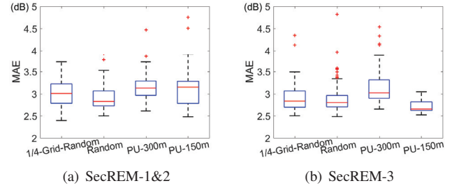
Fig. 13. MAEs of SecREM-1&2 and 3 vs. locations of false measurements.
