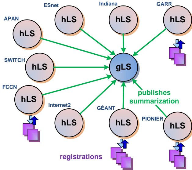
Figure 5. Simulated distributed test bed for validating the summarization algorithm.
