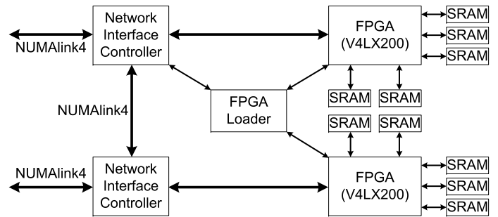
(b) RASC RC100 FPGA blade architecture
