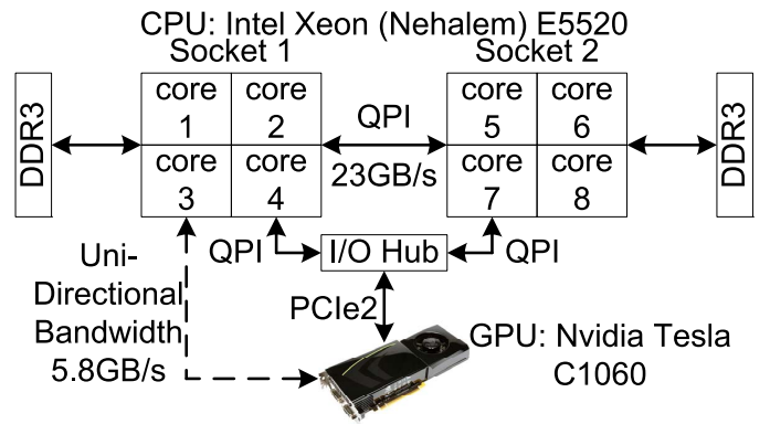
Fig. 5. The heterogeneous CPU-GPU board
