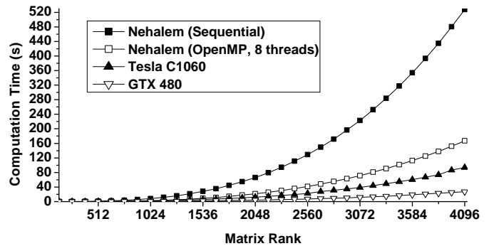
Fig. 7. Performance scalability of vector-based implementations of Hessenberg reduction
