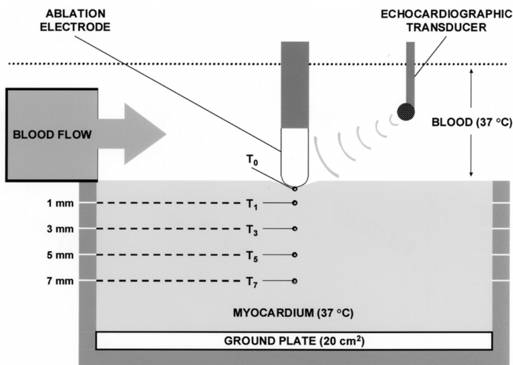
Fig. 2. Schematic of in vitro ablation system.
