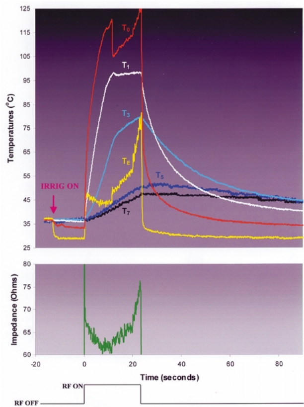
Fig. 6. Typical trial in experimental group 4, internal irrigation design, blood flow = 0.26 m/sec. Note that T_0 rises rapidly to boiling, at which point it abruptly deflects downward. This deflection was coincident with the sudden elaboration of echocardiographic bubbles at the electrode–endocardial interface and an audible “pop,” not associated with a significant impedance rise. Trials stopped at this instant (data not shown) showed displacement of the interface thermocouple to a site adjacent to the interface. After a few seconds, T_0 resumes its rise, but at a much slower rate. Note that despite the evidence of electrode–endocardial interfacial boiling, continued RF application is associated with progressive rise in intramural temperatures. Impedance rise subsequently reaches 10 ohms, precipitating premature generator shutoff.
