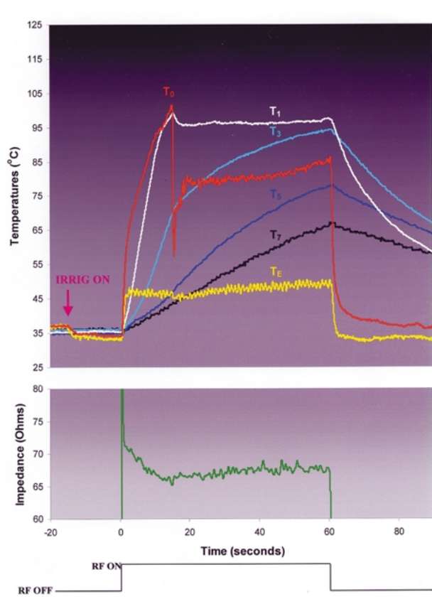
Fig. 7. Typical trial in experimental group 6, showerhead irrigation design, blood flow = 0.26 m/sec.
