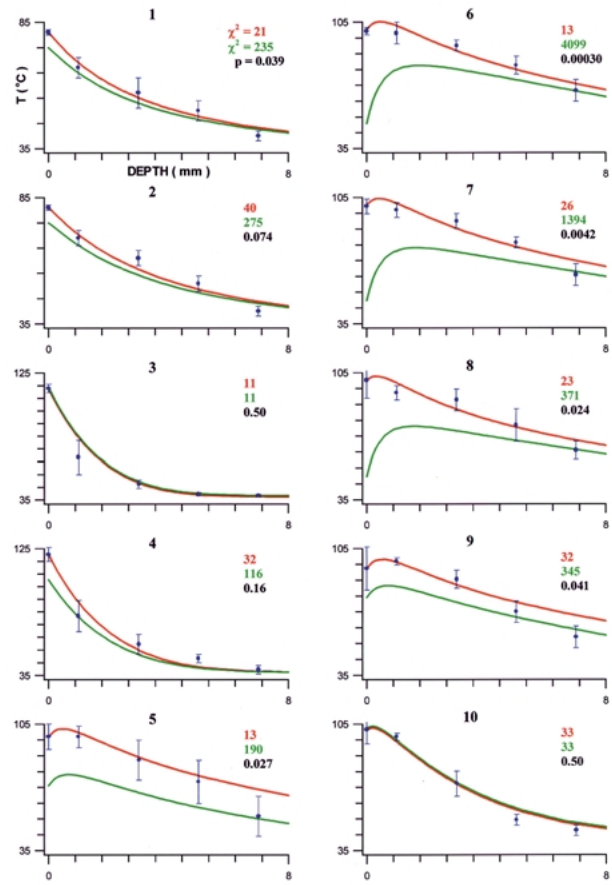
Fig. 4. Finite element simulation results, separated by experimental group (labeled on top of each graph): FEM 2 (assuming T_0 predicts intramyocardial temperatures) in red; FEM 1 (assuming T_E predicts intramyocardial temperatures) in green. The data points (mean temperature) with error bars (standard deviation) represent in vitro data. The chi-square value, quantifying the agreement between FEM and in vitro data, is shown in the corresponding color. A variance ratio test was performed between the chi-square values of FEM 1 and FEM 2; the resulting P value indicates whether FEM 2 agreed with the in vitro data significantly better than FEM 1.
