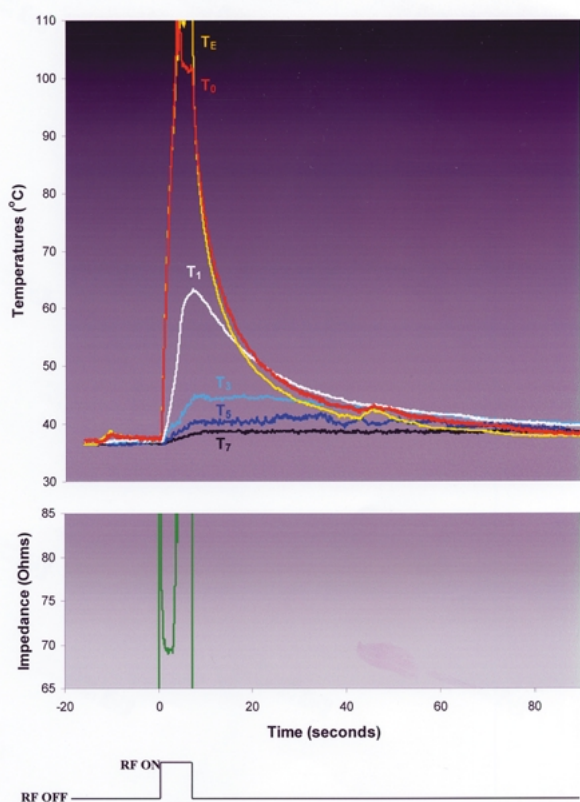
Fig. 5. Typical trial from experimental Group 3: no irrigation, no blood flow, RF power was fixed at 50 Watts.
