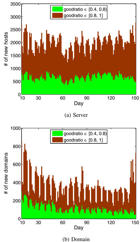
Fig. 1. Number of newly-appeared senders per day
