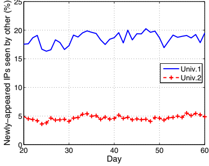
Fig. 5. Percentage of newly-appeared IP addresses that have been recorded by the other university over all newly-appeared IP addresses in daily logs
