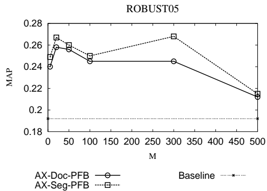
Figure 5: Performance Sensitivity (Num of Docs)
