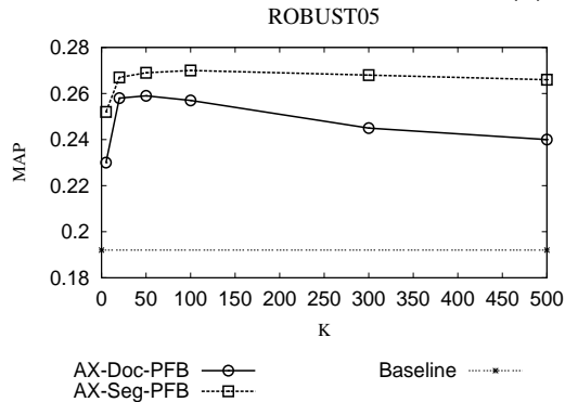
Figure 4: Performance Sensitivity (Num of Terms)
