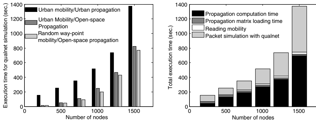
Fig. 17. Simulation execution time. The left-hand frame shows the simulation execution time for three simulation techniques. The right-hand plot shows a break-down of the execution time when realistic propagation is included. The propagation computation time includes the time to identify which floor tile a node is nearest and the time to look-up the propagation between nodes from the propagation matrix.
