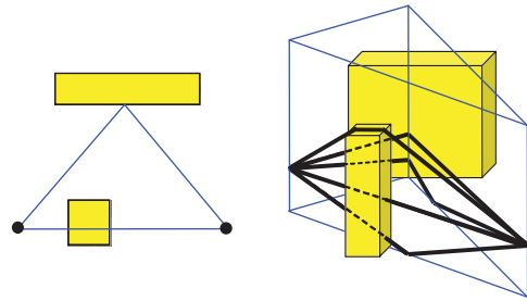
Fig. 10. Left: a top-view of the scene on the right. The lines shown are found from 2-D ray-tracing. Right: Two vertical plane paths (found from 2-D ray-tracing) and five ray paths.
