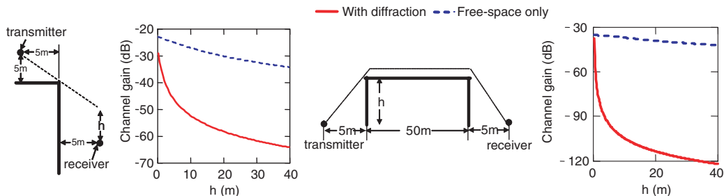
Fig. 7. Diffraction around a corner (left) and over a building (right). The left-hand frame and second from the right frame show side views of the simulated scenario. The other frames show the attenuation as a function of h . As h increases, the signal strength decreases. The dashed lines show the signal strength if the loss was only due to free-space propagation while the solid line shows the signal strength when the loss due to diffraction is also included.
