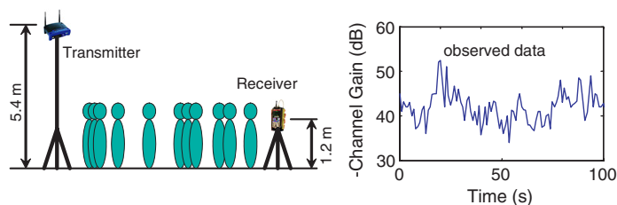
Fig. 8. Left, experimental setup for measuring the time-varying nature of propagation in a busy street in Philadelphia. Right, an observed time-series of the channel gain.
