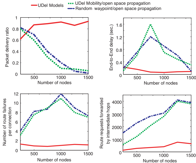
Fig. 16. Performance of a network under different types of mobility and propagation.
