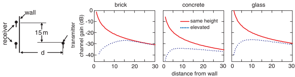
Fig. 4. Transmission through a wall. The left-hand frame shows a side-view of the simulated scenario. The right-hand frames depict the attenuation of the signal when transmitted through walls of different kinds of materials. It also depicts the nature of attenuation due to relative heights of the transmitter and the receiver.
