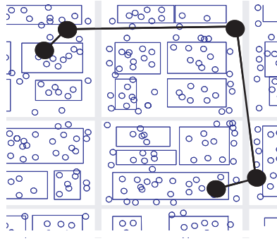
Fig. 3. Routing in an urban ad hoc network. The source and destination are inside of two different buildings. The shortest hop path travels along the road, it does not follow the shortest geometric route (i.e., a straight line).
