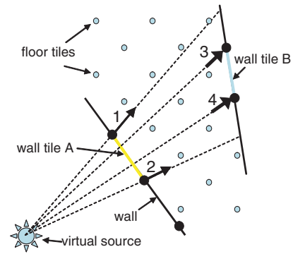
Fig. 11. Beam tracing. Suppose a beam strikes the wall tile marked A. The reflection of this beam is modeled as a beam emanating from the virtual source as shown. This beam is between and is defined by the two rays marked 1 and 2. These rays are used to select the floor tile ray-neighbors that this beam strikes (since ray-neighbors are precomputed, this selection is computationally efficient). Similarly, the rays 1 and 2 are used to select the set of A's wall tile ray-neighbors that the beam strikes. One such wall tile is shown in the upper right and is marked B. The beam that strikes tile B is defined by the rays marked 3 and 4. These rays define the beam that is transmitted through tile B and can be used to find the beam that is reflected off of B. This process of reflection and transmission is repeated until the beam's strength is small enough that it can be neglected (e.g., -110 dB).
