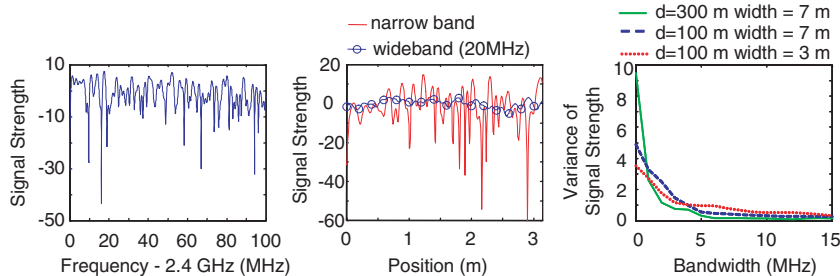
Fig. 6. Fast fading in narrow band and wide band communication scenarios. Left: the signal strength as a function of frequency for a narrow band signal propagating down an urban canyon. Middle: signal strength of a narrow and wide band signal as a function of receiver position perturbation when propagating down an urban canyon. Right: variance in signal strength due to change in receiver position as a function of bandwidth for when propagating down a urban canyon as shown in Fig. 5.
