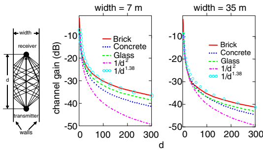
Fig. 5. Propagation down a street. The left-hand frame shows a top view of the simulated scenario. The right-hand frames depict the effect of propagation down an urban canyon for different wall materials, different attenuation exponents, and for the free space.
