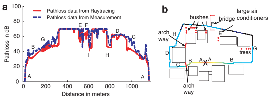
Fig. 12. Observed and estimated path loss in the campus environment.
