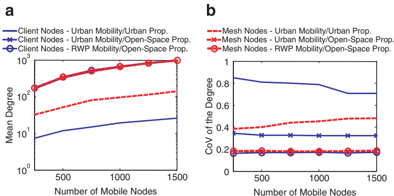
Fig. 15. Statistics of degree distribution in random way-point with open-space propagation, urban mobility with open-space propagation and urban mobility with realistic urban propagation. The mesh infrastructure nodes are fixed on top of streetlights, while the client nodes are mobile. The coefficient of variance (CoV) is the standard deviation divided by the mean.
