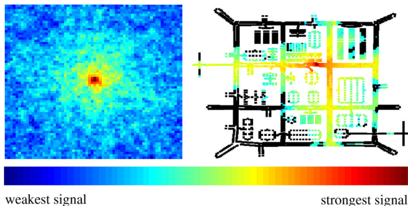
Fig. 2. Left, channel gain generated by a correlated lognormal model. Right, channel gains generated by ray-tracing in an urban area. The rectangle shapes are buildings and the shaded boxes inside the rectangles represent channel gain to locations on the first floor of the building. In both the left and right frames, the star marks the location of the transmitter.
