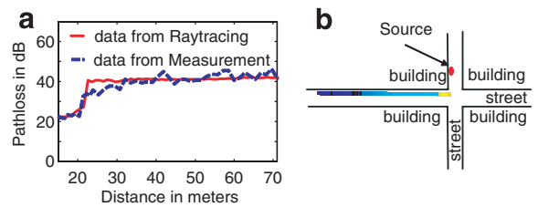
Fig. 13. Observed and estimated path loss at an intersection in Philadelphia.
