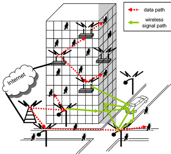
Fig. 1. Urban mesh networks are composed of wireless links between infrastructure nodes and wireless links between infrastructure and mobile clients. Both types of nodes may be indoors or outdoors and may be elevated or at street level. Communication between mobile clients and the Internet is provided via multiple wireless hops over the infrastructure (dotted lines). Many types of signal propagation are relevant. In the figure above, the signals that reach the car are impacted by diffraction around the corner of the building, propagation through the interior of the building, transmission through an exterior building wall, and reflections off of a building and off of the ground.
