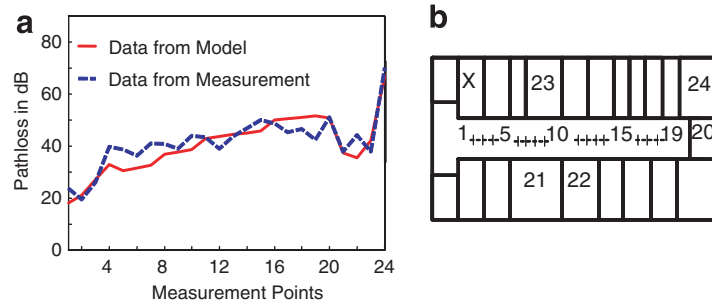
Fig. 14. Observed and estimated path loss in an indoor environment. The measurement points shown on the x-axis correspond to the numbered locations in the map. The map is of the third floor of Evans Hall in University of Delaware campus.
