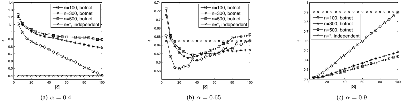
Fig. 2. Performance comparison of independent and botnet methods in spam distribution at different \alpha in terms of the single objective f .
