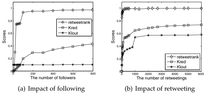
Fig. 6. Manipulating digital influence by following and retweeting.
