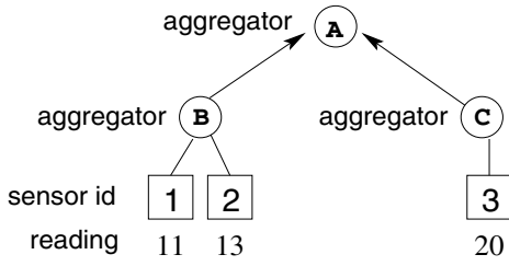
Figure 3: Example for hierarchical aggregators.
