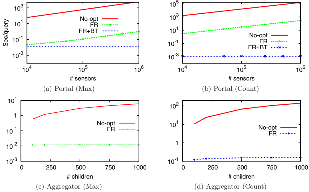
Figure 7: Per-query computational load on portal and aggregator. “No-opt” means no optimizations, “FR” means folded rolling, and “BT” means B-Tree.
