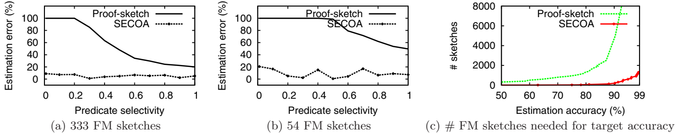
Figure 8: Comparing SECOA with proof-sketches. (c) uses a selectivity of 1.
