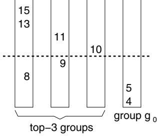
Figure 6: An example with 8 sensors. The numbers are sensor readings. For all sensors with readings below 10, regardless of which group they are classified into, the final result (i.e., 15, 11, and 10) will not be affected.
