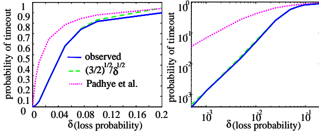
Figure 2. Probability of Timeout. The solid blue line represents the observed probability of a flow being in timeout. The dashed green line is the model's estimate of this probability. Note that these two lines nearly coincide. The third curve is the relationship derived from [11].
