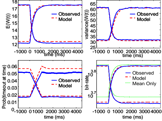
Figure 5. These figures are similar to the ones shown in Figure 4. However, here two sets of dynamics are shown, the loss probability jumping from 0.1% to 1% and falling from 1% to 0.1%. In both cases, the changes occur at t = 0 .
