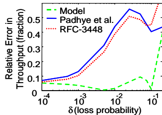
Figure 3. Relative Error of Predicted Throughput. Note that an error fraction of 0.5 implies a 50% error.
