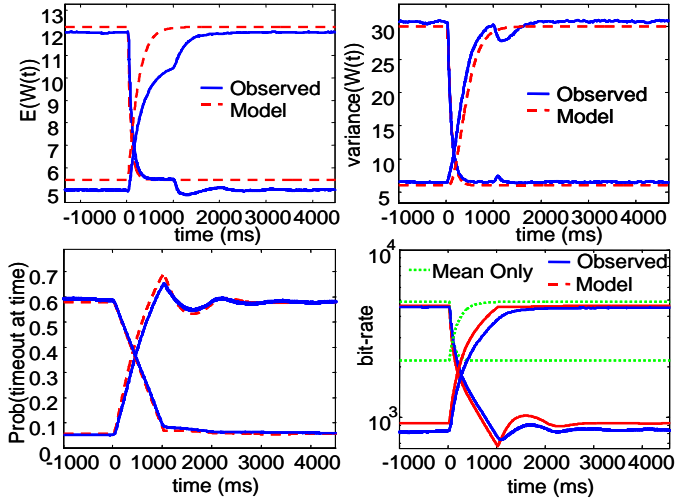
Figure 6. Validation of the Model. These figures are near identical to Figure 5, however, here the loss probability jumps between 1% and 5%.
