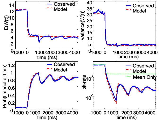
Figure 4. Simulation and modeling of a jump in loss probability from 1% to 10%. The jump occurred at t = 0 . The solid blue curves show the observed and the dashed red curves shows the model. In the lower right, the dotted green indicates the bit-rate if only the mean size of the congestion window is used (i.e., the dashed red curve in the upper left). Note the units of the bit-rate is in 1000 bps.
