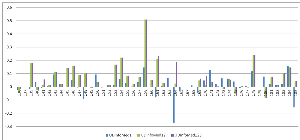
Figure 1 Improvement of each run compared with median (InfAP)
