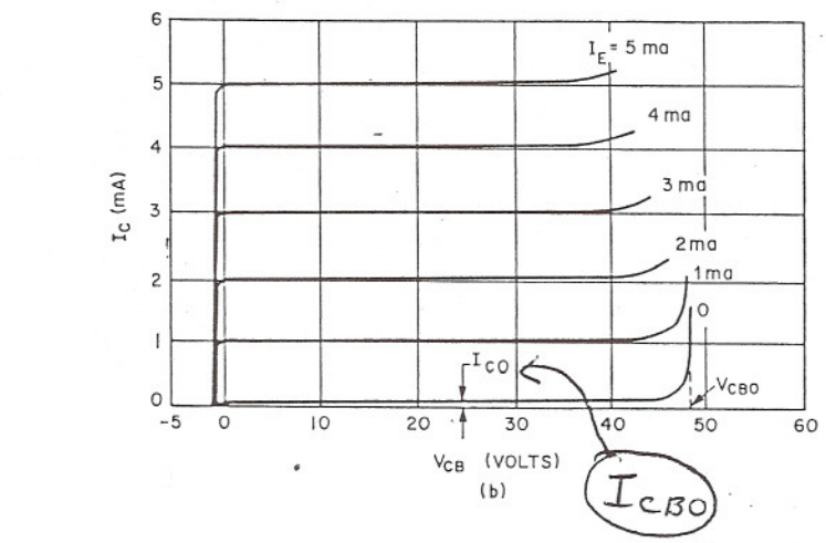
output characteristic of a typical p-n-p transistor in common-base configuration.
