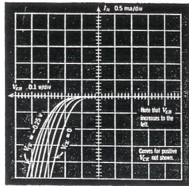
Common-emitter transistor characteristics, showing the comparison between actual curves (left) and the predictions of the Ebers-Moll two-diode model (right).
