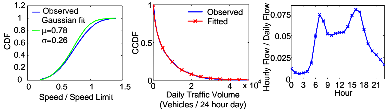
Fig. 10. Left, Cumulative distribution function (CDF) of the vehicle speed in urban areas and a fitted Gaussian CDF. Middle, complementary cumulative distribution function of the vehicle traffic volumes on San Francisco streets. Right, ratio of hourly volume to daily volume.
