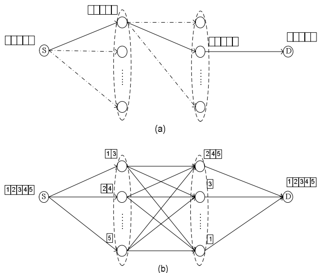
Fig. 1: (a) Selective OFDM Relaying in a 3-hop network, i.e., at each hop the relay with the largest combined SNR is selected out of L relays to forward the entire OFDM block; (b) Selective OFDMA Relaying in a 3-hop network, i.e., the best relay is selected for each subcarrier at each hop. Each subcarrier chooses the path independently.
