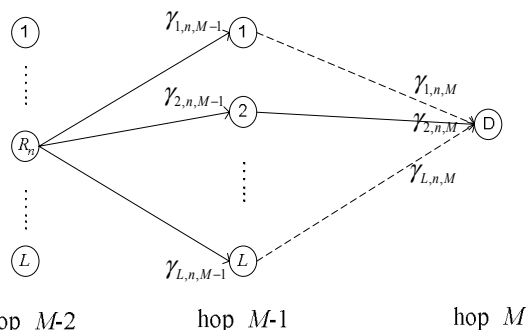
Fig. 2: Relay selection for subcarrier n at hop M-1 . The relay with the largest \min(\gamma_{l,n,M-1}, \gamma_{l,n,M}) , instead of \gamma_{l,n,M-1} , is selected.
