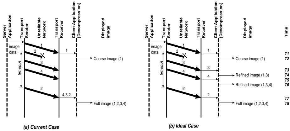
Fig. 2. Progressive Image Transmission over a Lossy Network (2 Cases)
