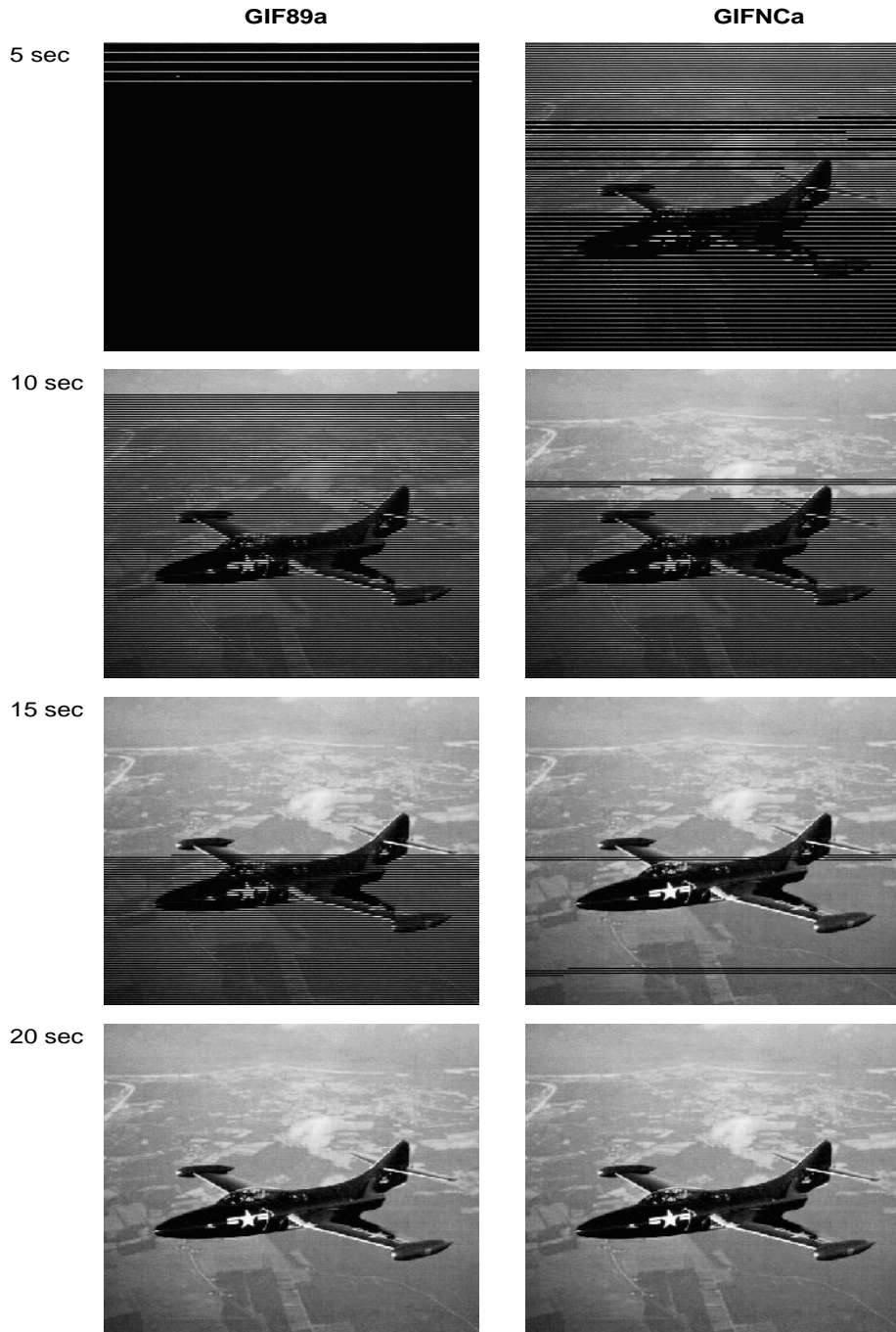
Fig. 5. Sequence of GIF89a and GIFNCa Images at 10% Loss
