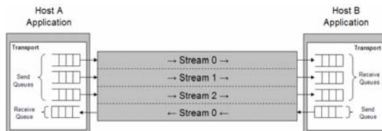
Figure 2: Use of streams within an SCTP association
