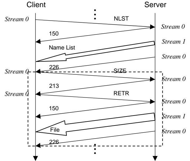
Figure 4: FTP over SCTP-MS
