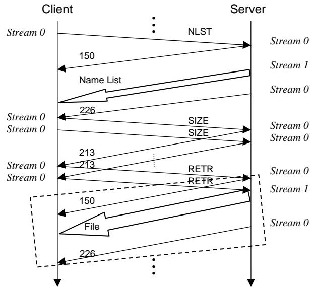
Figure 5: FTP over SCTP-MS-CP
