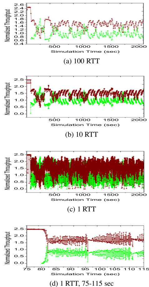
Fig. 7. Throughput of SCTP (red or dark color) followed by TCPS (green or light color), for different time intervals. (For interpretation of the references to colour in this figure legend, the reader is referred to the web version of this article.)
