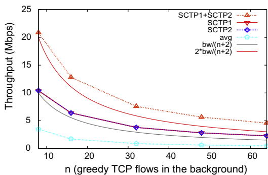
(b) two-SCTP
