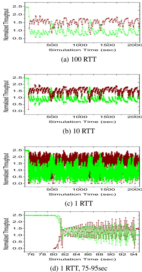
Fig. 8. Throughput of TCPS (green or light color) followed by SCTP (red or dark color), for different time intervals. (For interpretation of the references to colour in this figure legend, the reader is referred to the web version of this article.)
