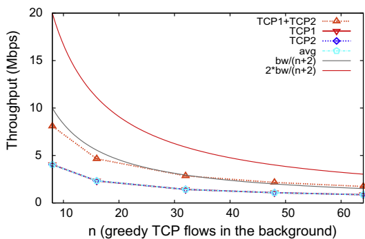
(a) two-TCP
