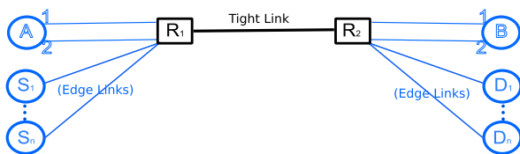
Fig. 9. Simulation topology for the TCP-friendliness of CMT.
