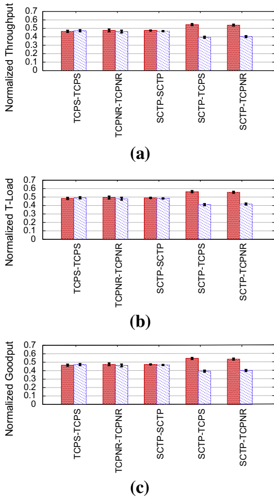
Fig. 4. (a) Normalized throughput, (b) T-Load, and (c) Goodput when both flows start at the same time.
