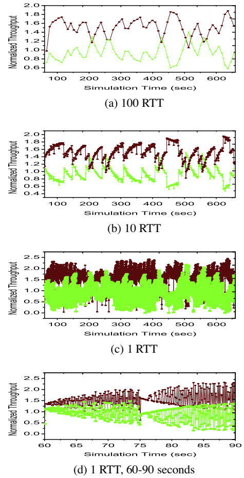
Fig. 5. Throughput of TCPS (green or light color) and SCTP (red or dark color), starting at the same time, for different time intervals. (For interpretation of the references to colour in this figure legend, the reader is referred to the web version of this article.)
