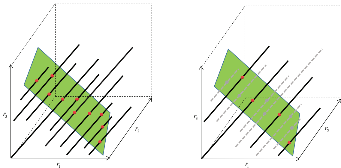
Fig. 3: Integer position representation with respect to three moduli.
