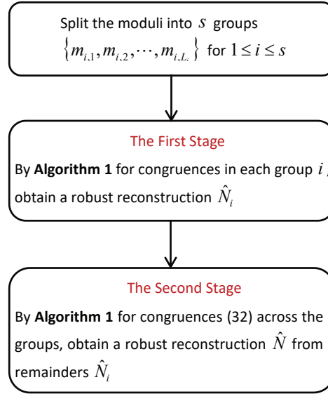
Fig. 1: Flowchart of the two-stage robust CRT algorithm.
