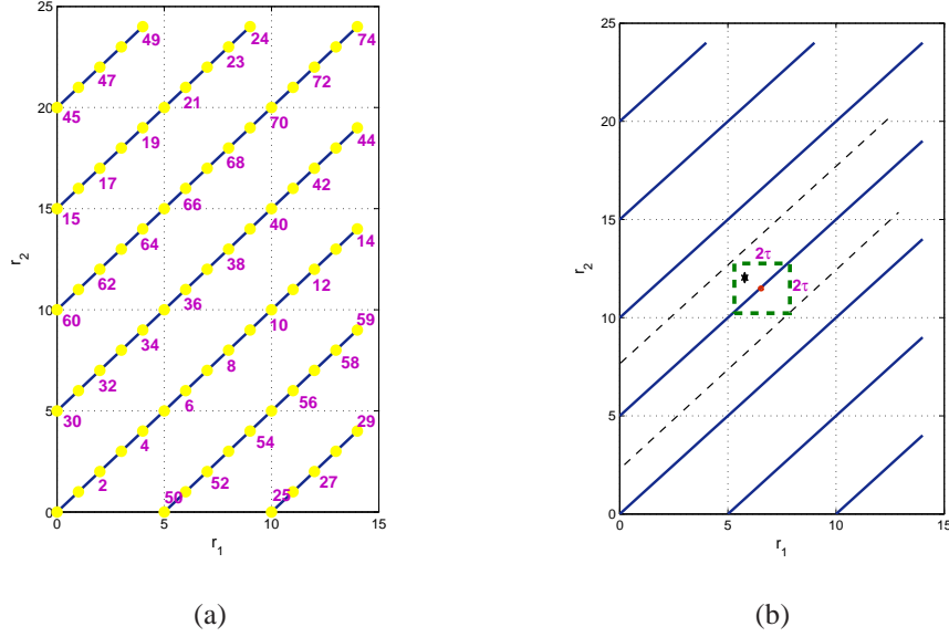
Fig. 2: (a) Integer position representation with respect to two moduli, m_1 = 15 and m_2 = 25 ; (b) The remainders of an integer with an error bound \tau .
