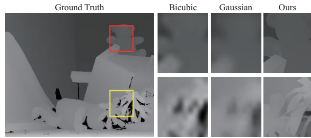
Fig. 5 Comparison of our method and other upsampling schemes on synthesis data. Both patches in the disparity map are upsampled from a resolution of 30 \times 25 to 450 \times 375 .
